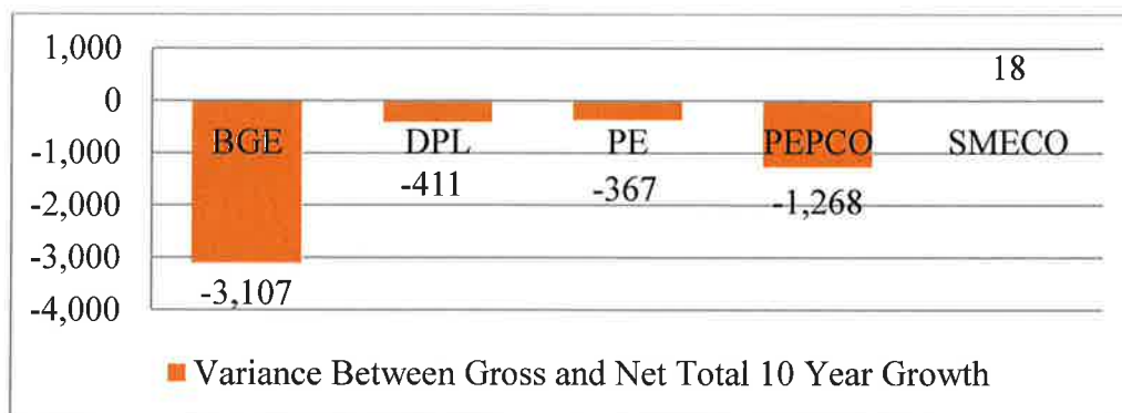
Figure 14 Impact of the Participating Utilities' DSM Programs on the Ten-Year Energy Sales Projections (MWh) 58
