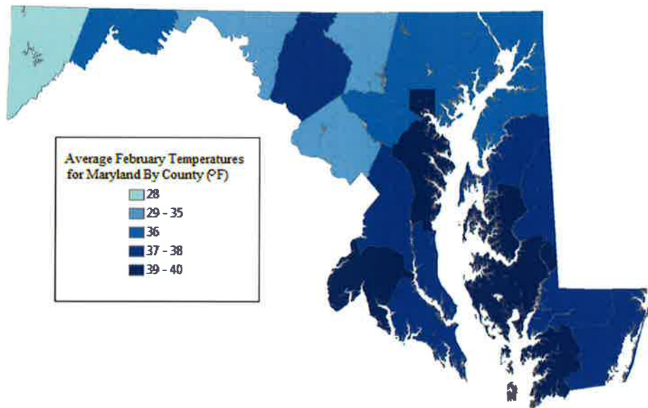
Figure 7 Average February Temperatures for Maryland 39
