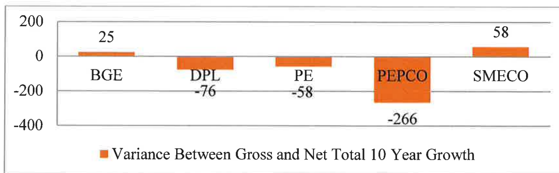
Figure 15 Impact of the Participating Utilities' DSM Programs on the Ten-Year Summer Peak Load (MW) 59
