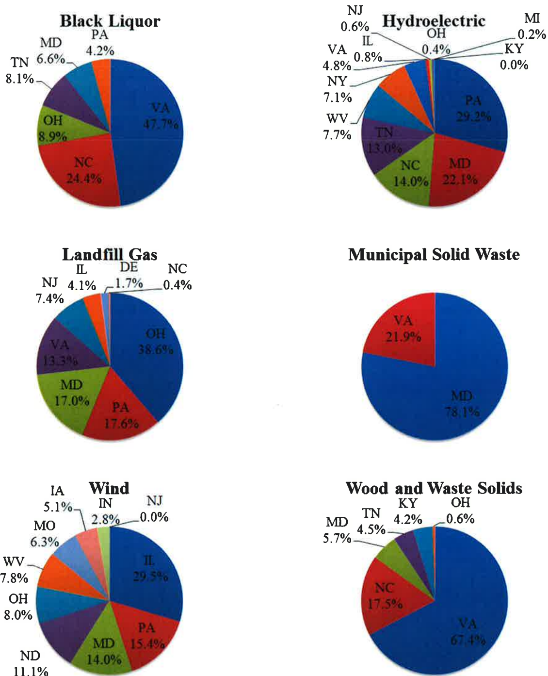
Figure 6: Percentage of RECs Generated in Each State, by Fuel (2017) 27
