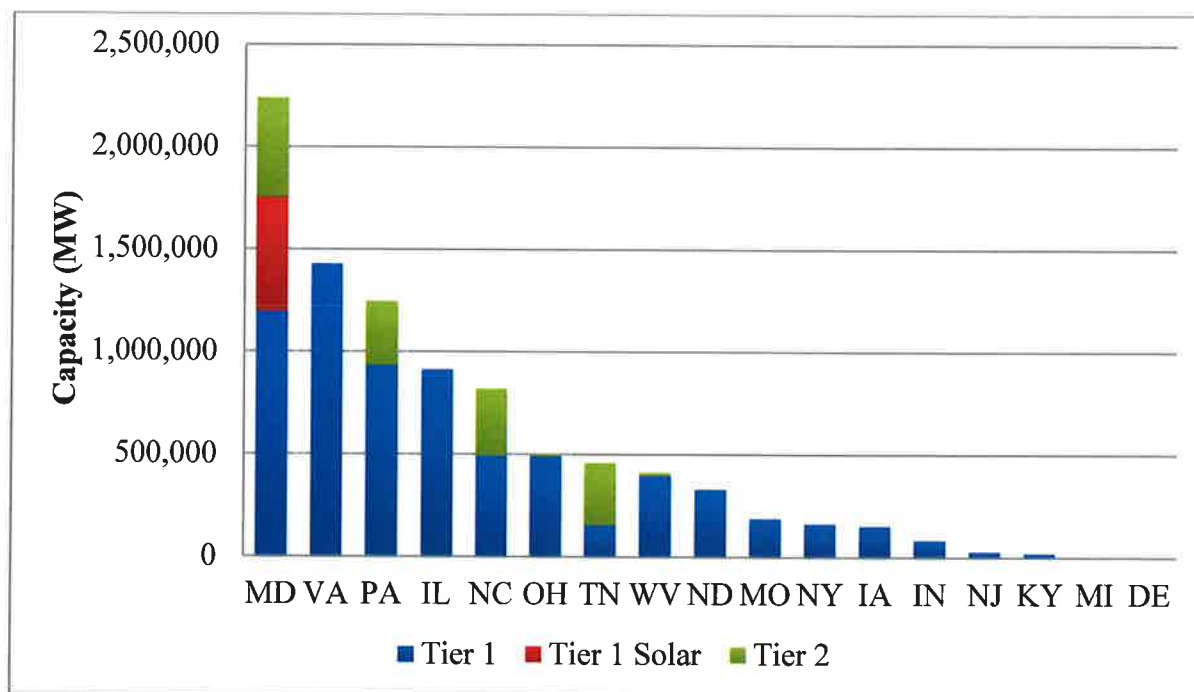
Figure 4: Number of RECs Retired by Facility Location (2017)
